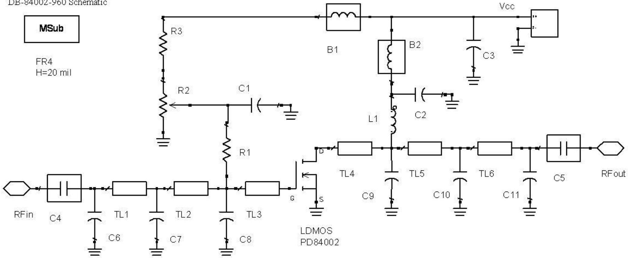
DB-84002-960 Schematic
